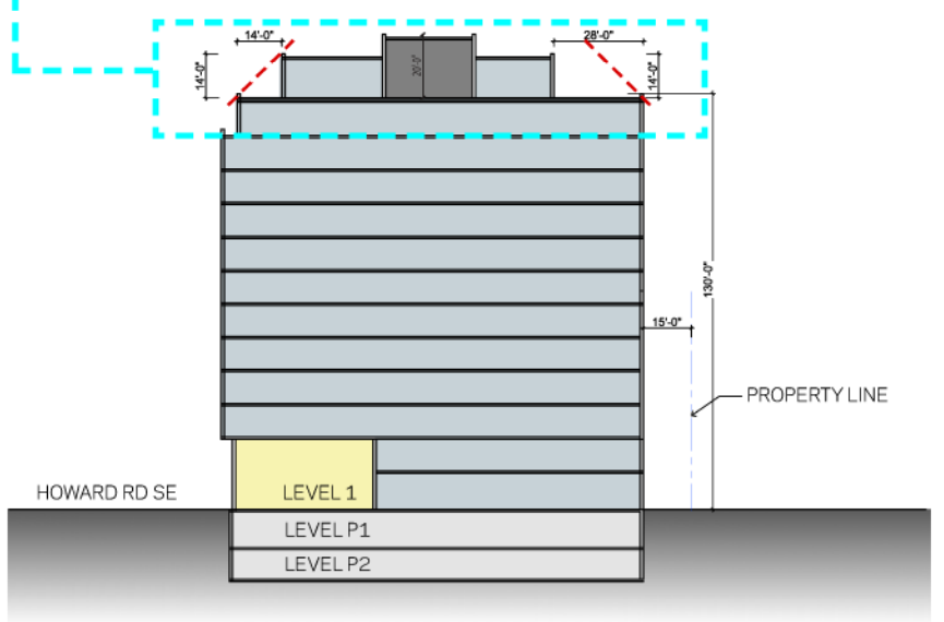
SECTION D-D'
