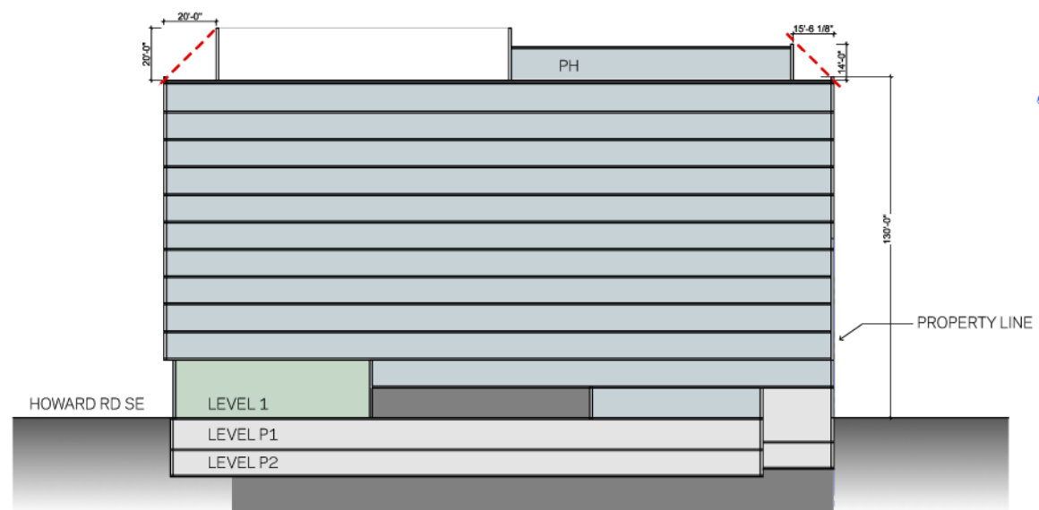
SECTION E-E'
