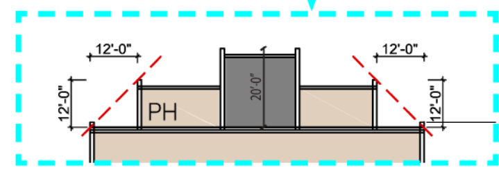
PENTHOUSE HEIGHTS
